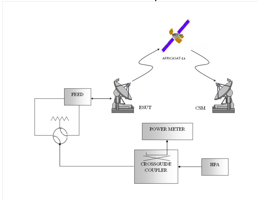
Figure 2: Transmit Antenna Side lobe Pattern / Cross-Polarization Isolation Measurement Setup
