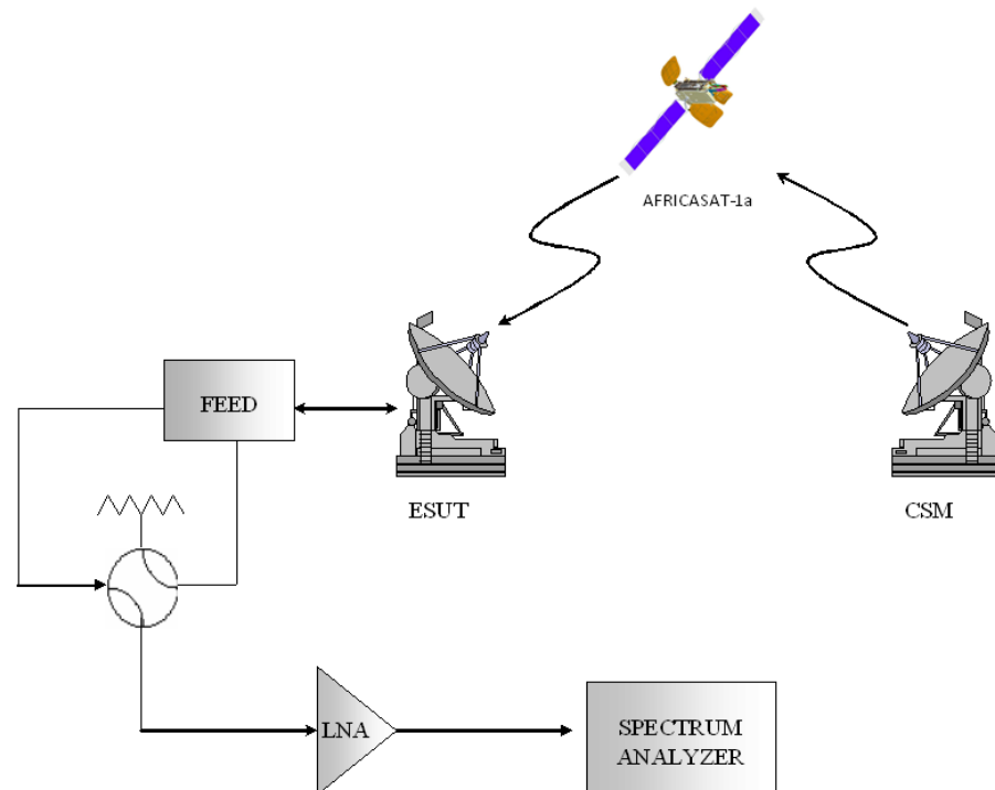
Figure 1: Antenna Pointing / Receive Cross-Polarization Isolation Measurement Setup
