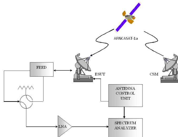
Figure 3: Receive Antenna Side lobe Pattern Measurement Setup
