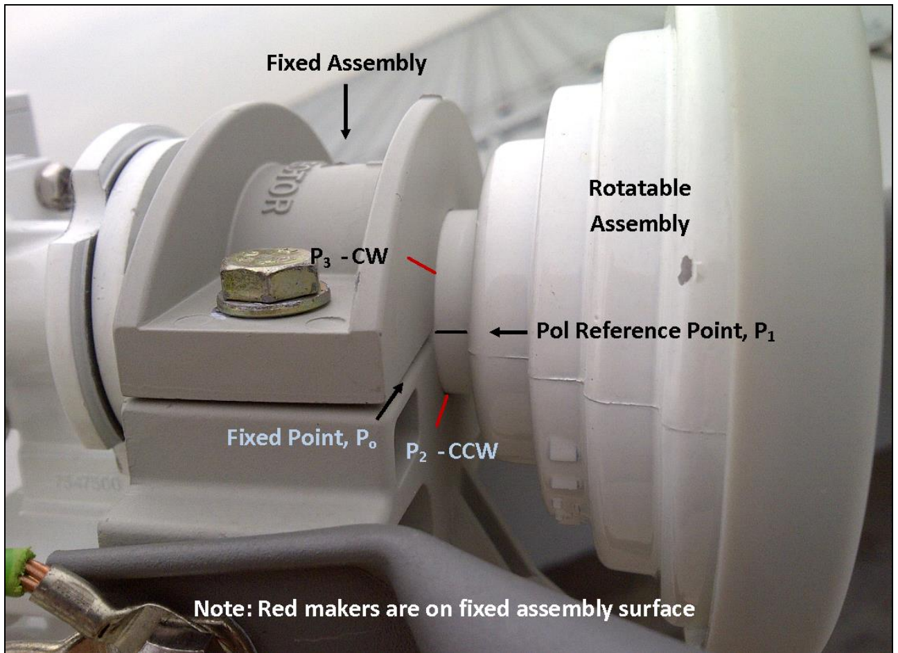
Figure 3: Point positions for polarizer optimization
