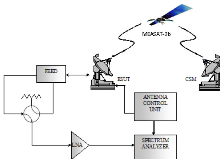
Figure 4: Receive Antenna Side lobe Pattern Measurement Setup
